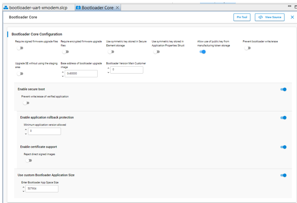
Figure 3.25. Bootloader Core configuration for Certificate-based Secure Boot
