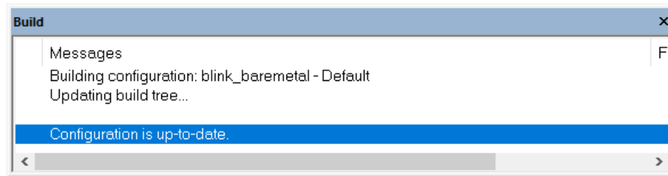
Figure 4.12. Build messages
