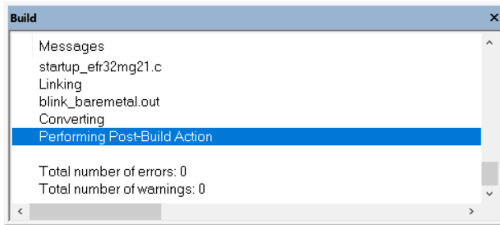
Figure 4.11. Build messages
