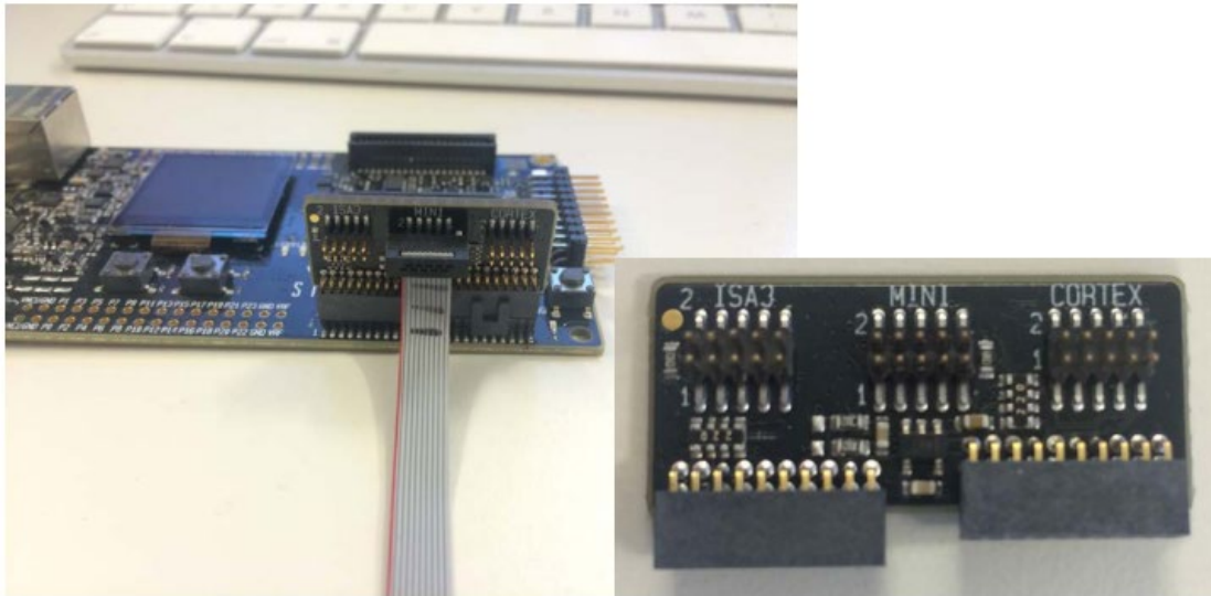
Figure 2.2. Simplicity Debug Adapter Exposing PTI Signals on the Mini and Simplicity Connectors
